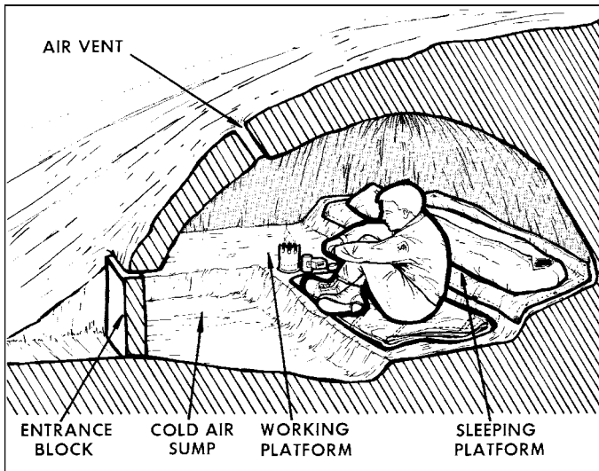
Figure VI-7. Snow Cave
