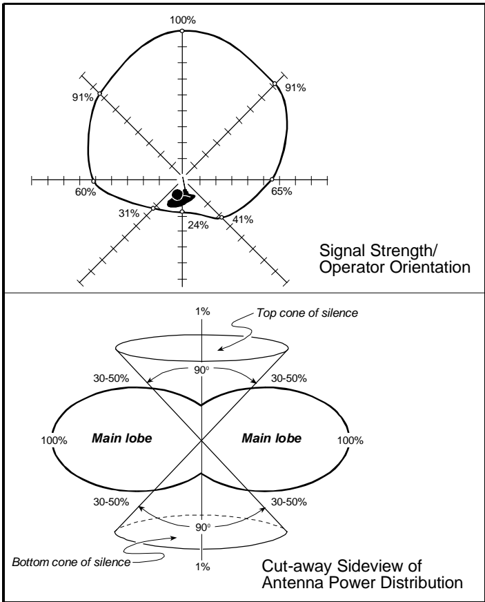
Figure III-1. Radio Transmission Characteristics
