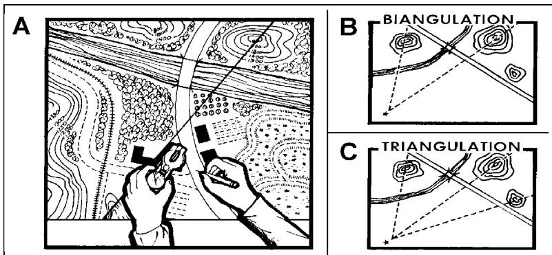
Figure II-7. Triangulation
