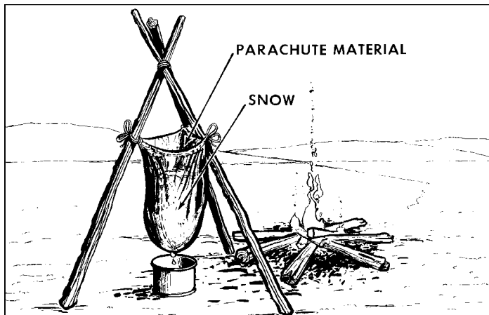
Figure VII-3. Water Generator
