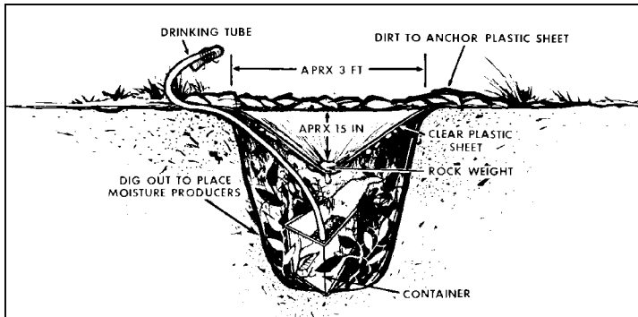
Figure VII-7. Solar Still
