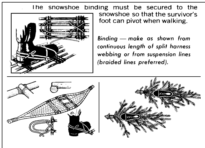
Figure II-10. Improvised Snowshoes
