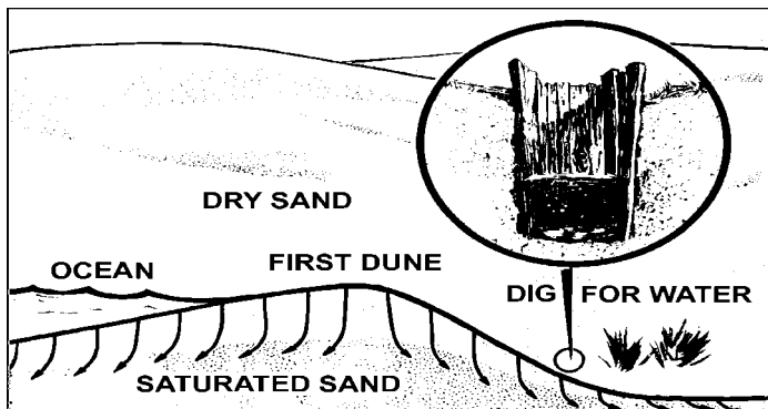
Figure VII-6. Beach Well
