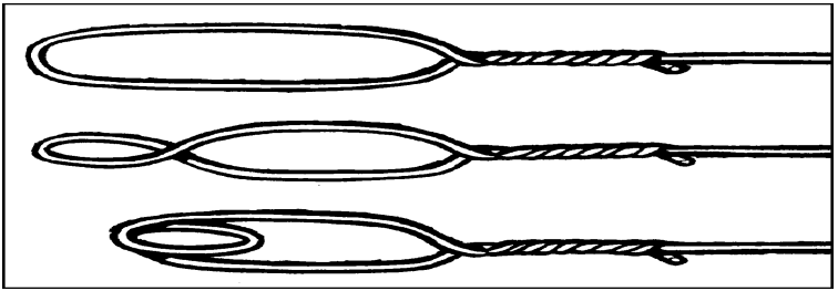
Figure VIII-3. Locking Loop
