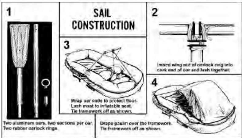
Figure II-12. Shade/Sail Construction
