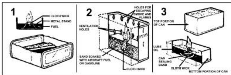
Figure VI-16. Improved Stove
