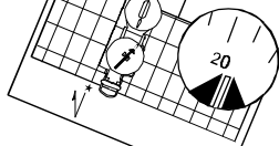
Figure II-5. Orienting a Map Using a True North-South Line
