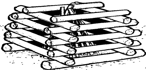
Figure VI-13. Log Cabin or Pyramid Fires
